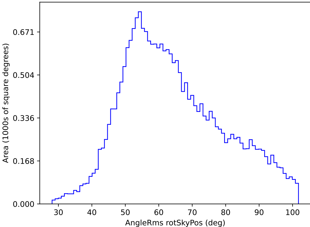
baseline_v2.0_10yrs All sky u band: AngleRms rotSkyPos
