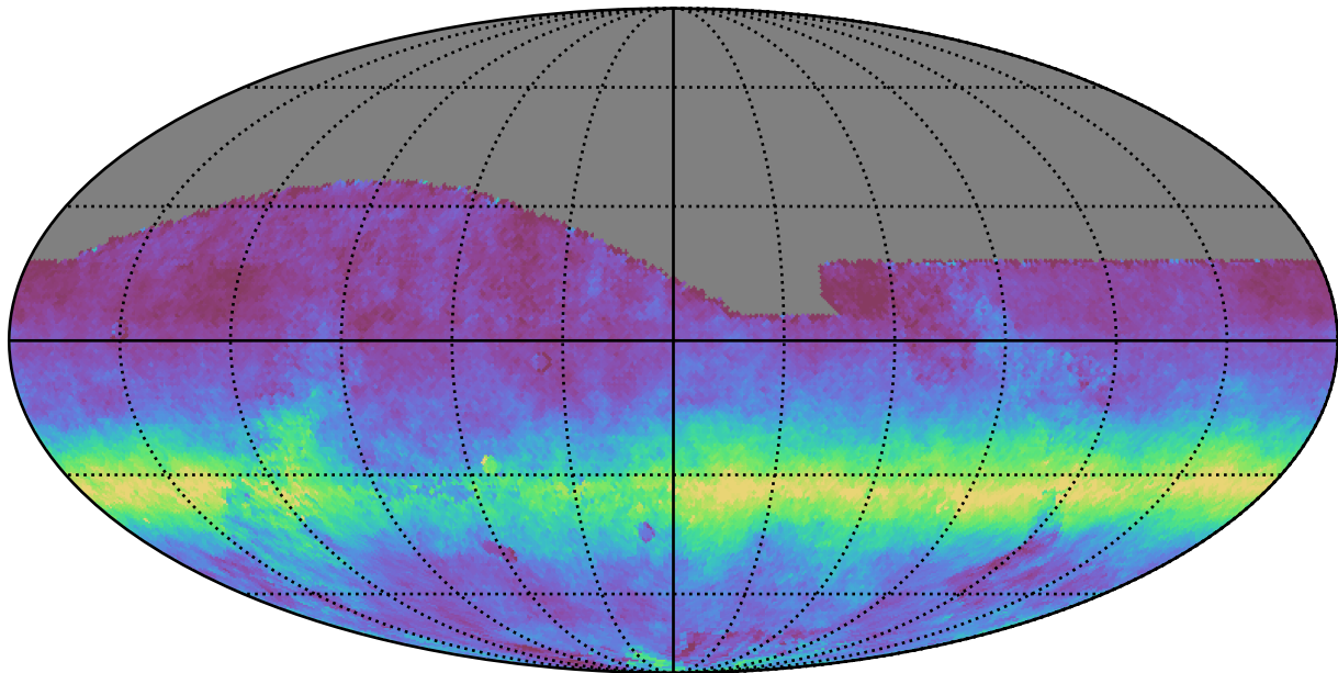
baseline_v2.0_10yrs All sky r band: AngleRms rotSkyPos
