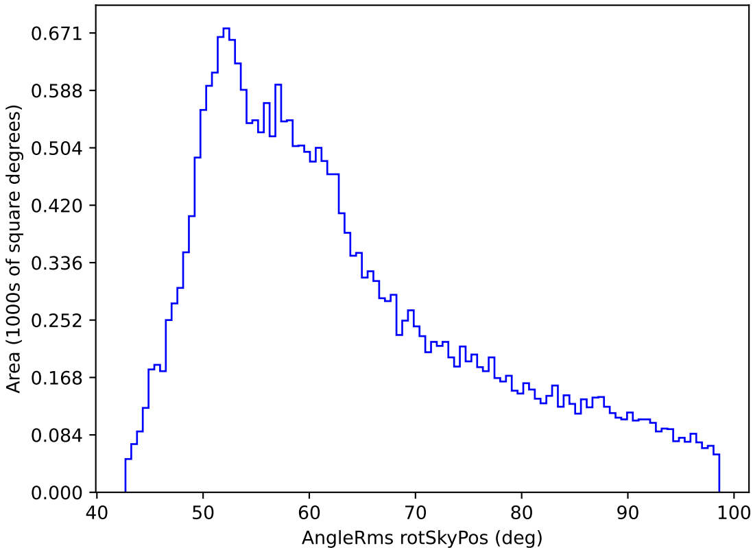
baseline_v2.0_10yrs All sky r band: AngleRms rotSkyPos
