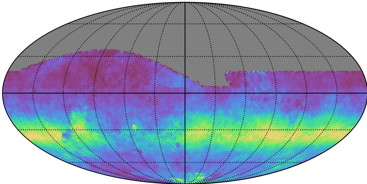
baseline_v2.0_10yrs All sky i band: AngleRms rotSkyPos
