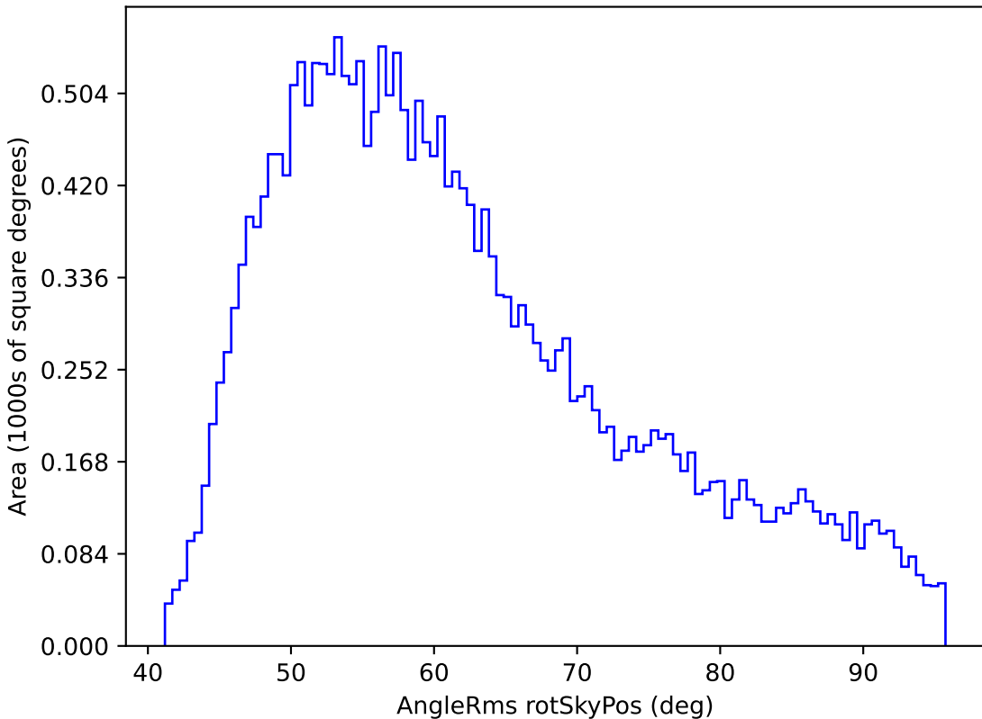
baseline_v2.0_10yrs All sky i band: AngleRms rotSkyPos
