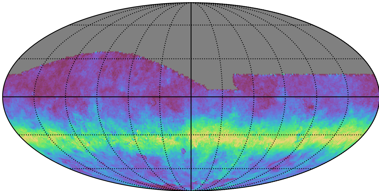
baseline_v2.0_10yrs All sky g band: AngleRms rotSkyPos
