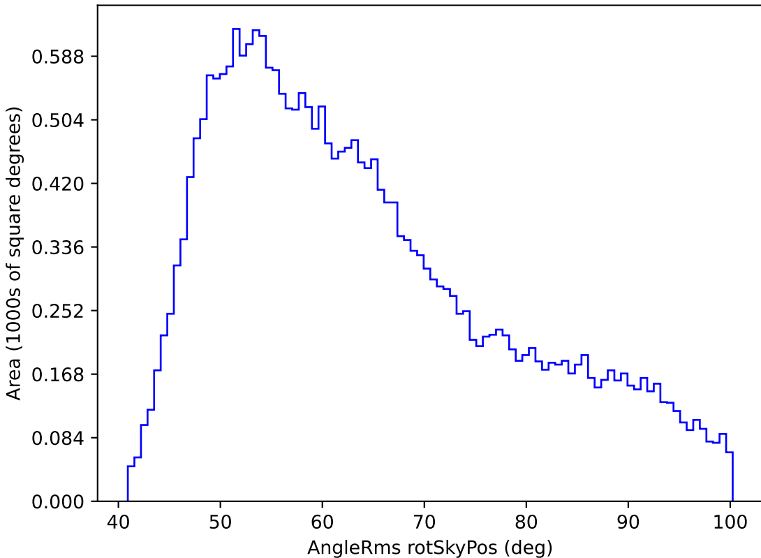
baseline_v2.0_10yrs All sky g band: AngleRms rotSkyPos
