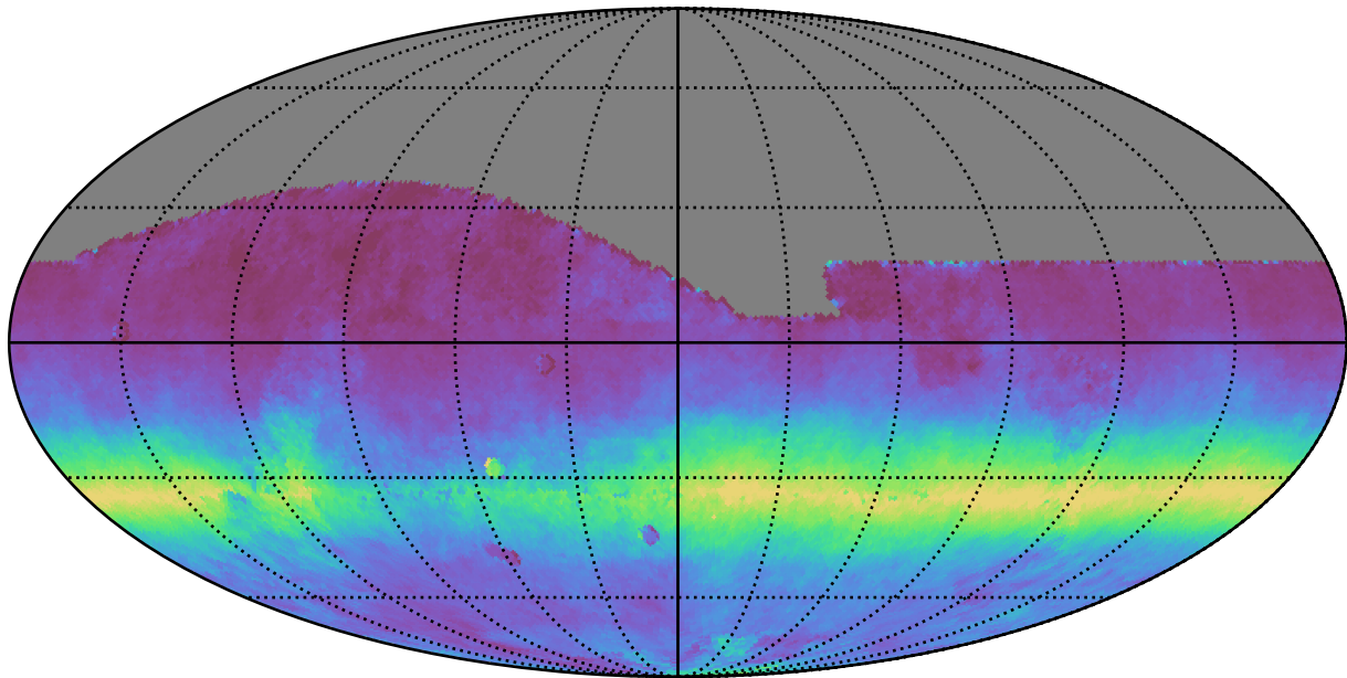
baseline_v2.0_10yrs All sky all bands: AngleRms rotSkyPos
