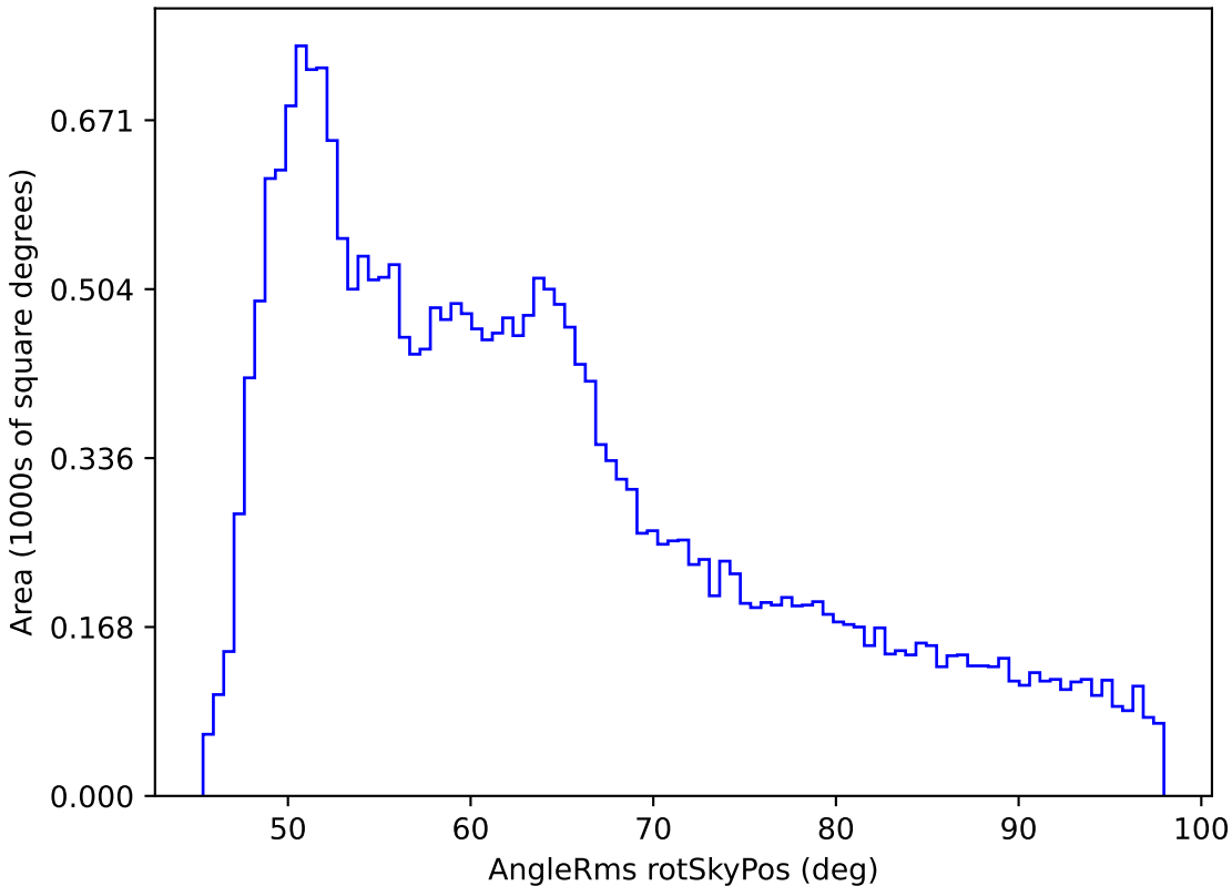
baseline_v2.0_10yrs All sky all bands: AngleRms rotSkyPos
