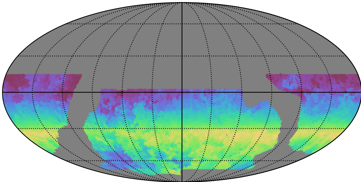
baseline_v2.0_10yrs WFD z band: AngleRange rotSkyPos
