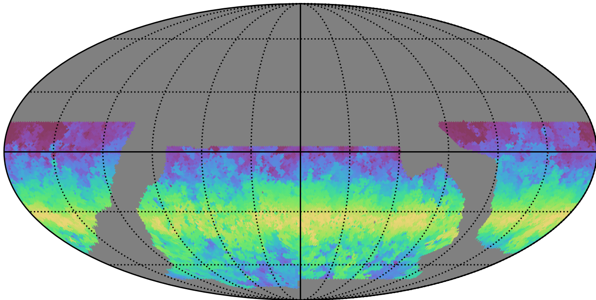
baseline_v2.0_10yrs WFD u band: AngleRange rotSkyPos
