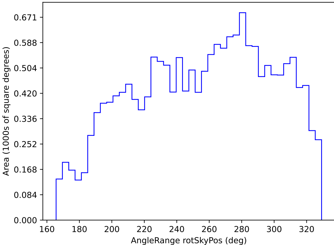
baseline_v2.0_10yrs WFD u band: AngleRange rotSkyPos
