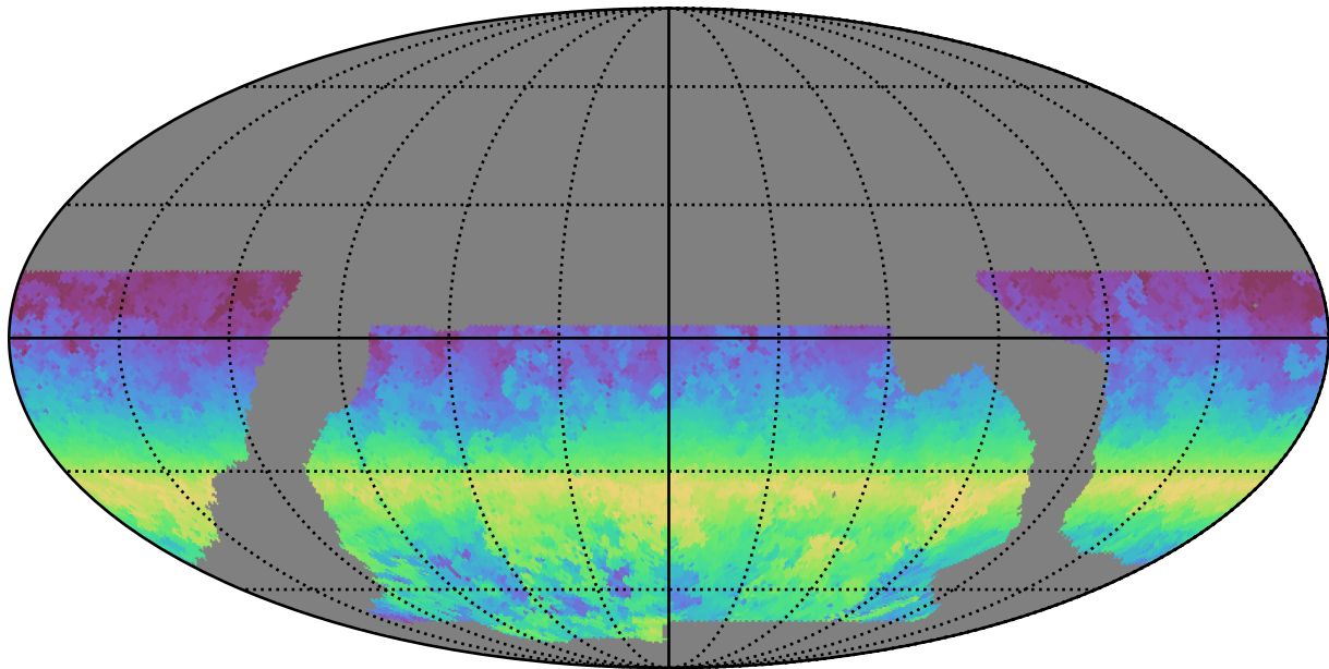
baseline_v2.0_10yrs WFD r band: AngleRange rotSkyPos
