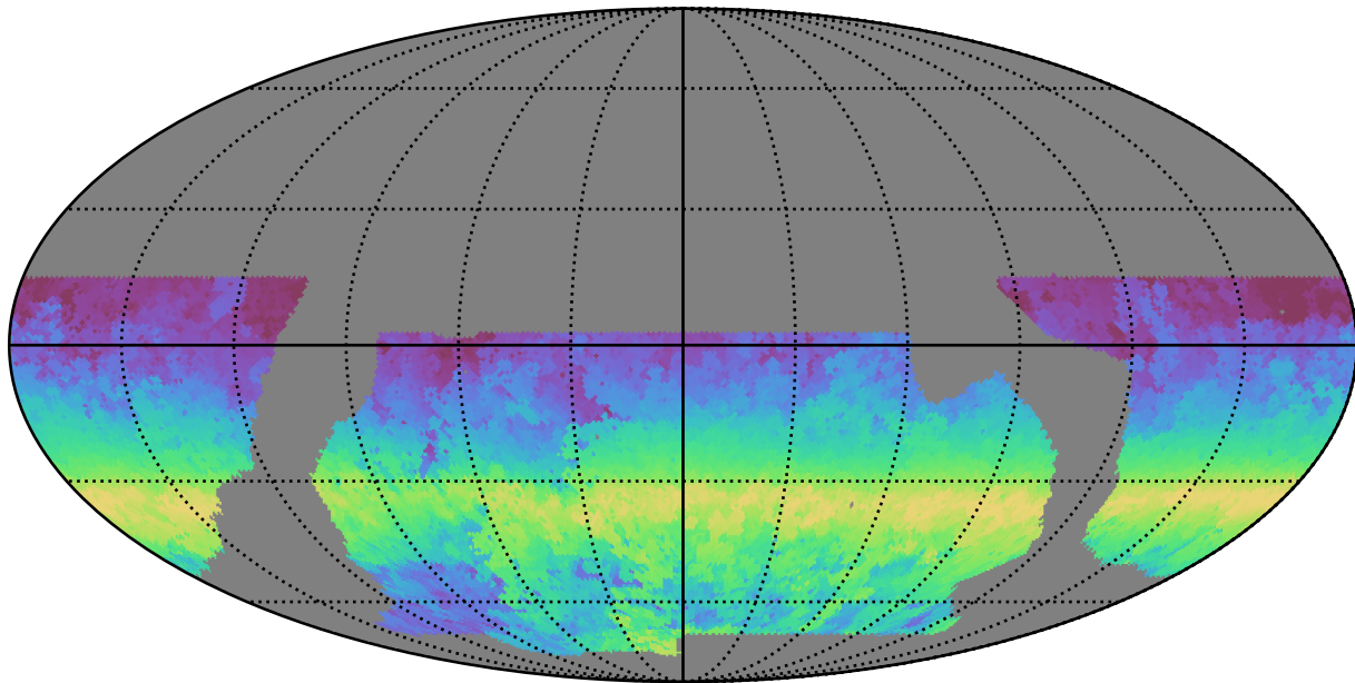
baseline_v2.0_10yrs WFD i band: AngleRange rotSkyPos
