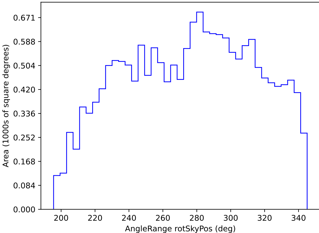
baseline_v2.0_10yrs WFD i band: AngleRange rotSkyPos
