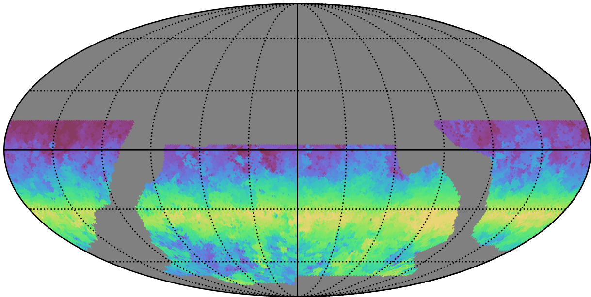
baseline_v2.0_10yrs WFD g band: AngleRange rotSkyPos
