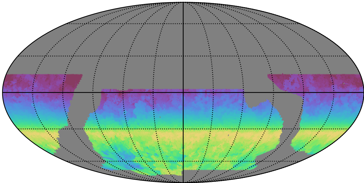
baseline_v2.0_10yrs WFD all bands: AngleRange rotSkyPos
