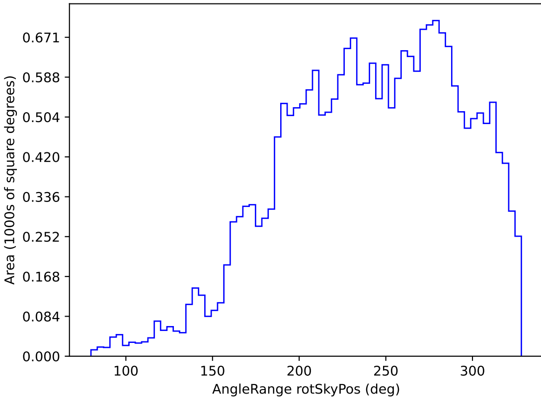
baseline_v2.0_10yrs All sky u band: AngleRange rotSkyPos
