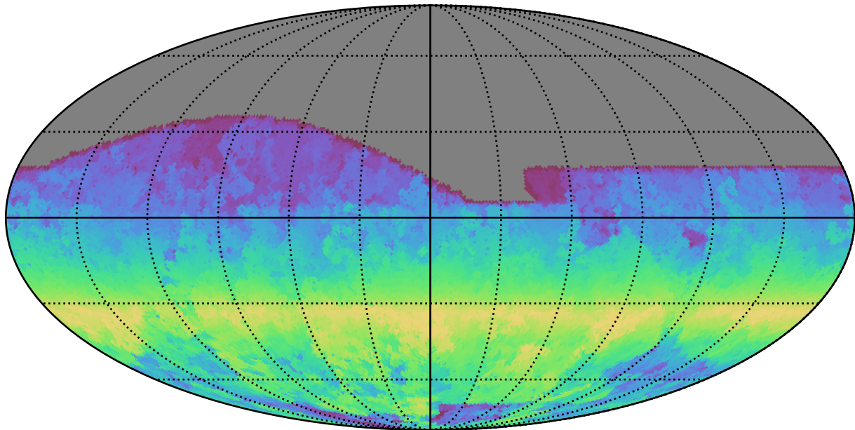
baseline_v2.0_10yrs All sky r band: AngleRange rotSkyPos
