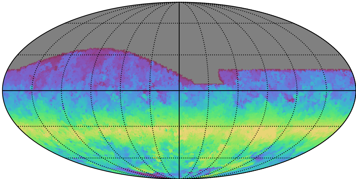
baseline_v2.0_10yrs All sky g band: AngleRange rotSkyPos
