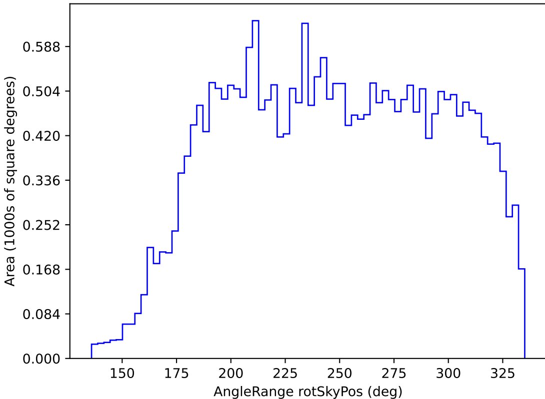
baseline_v2.0_10yrs All sky g band: AngleRange rotSkyPos
