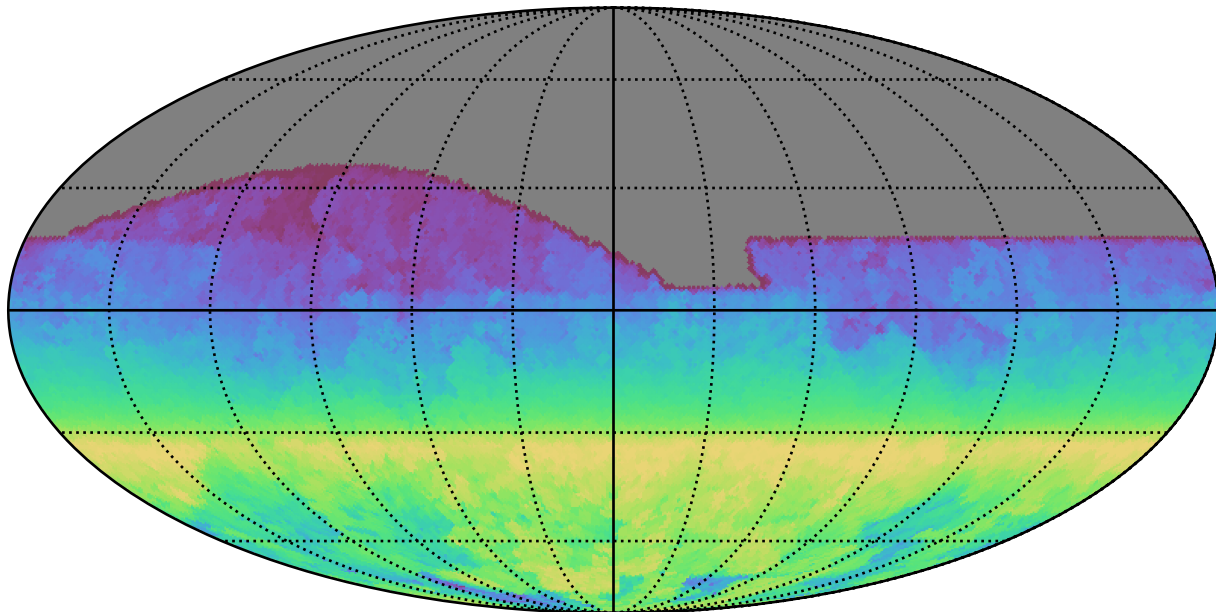
baseline_v2.0_10yrs All sky all bands: AngleRange rotSkyPos
