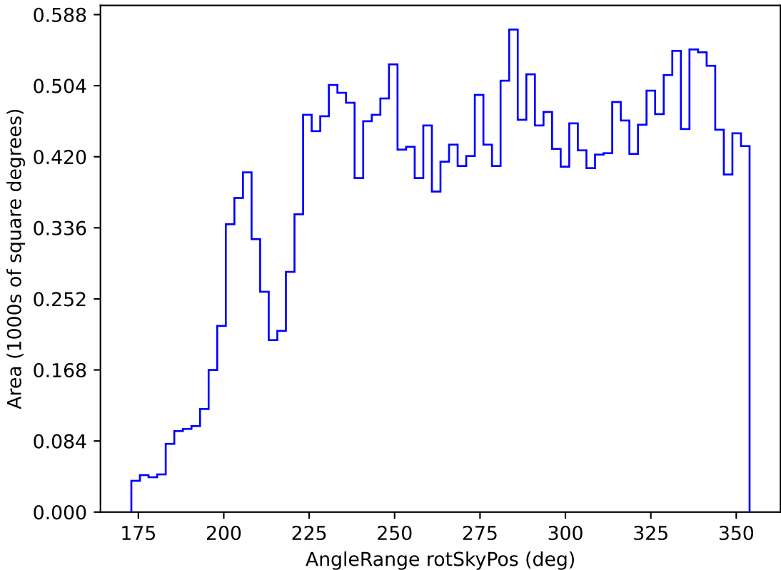
baseline_v2.0_10yrs All sky all bands: AngleRange rotSkyPos
