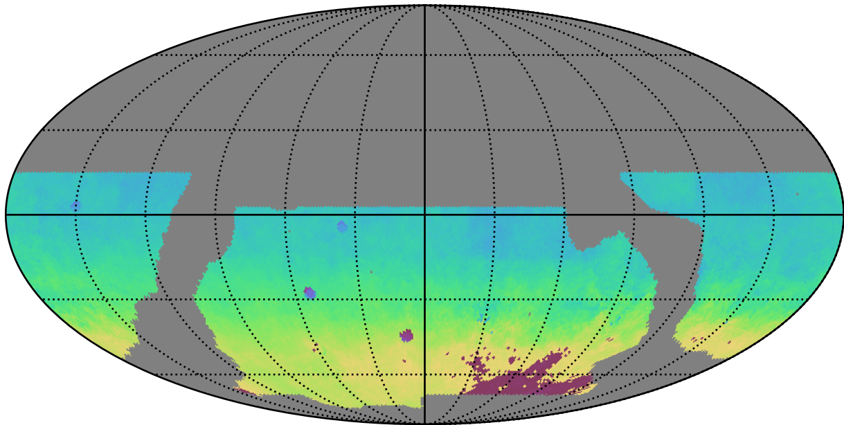
baseline_v2.0_10yrs WFD y band: AngleMean rotSkyPos
