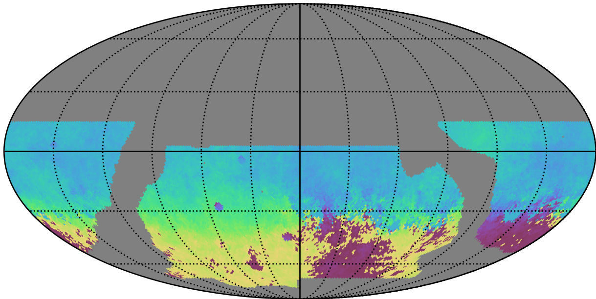
baseline_v2.0_10yrs WFD u band: AngleMean rotSkyPos
