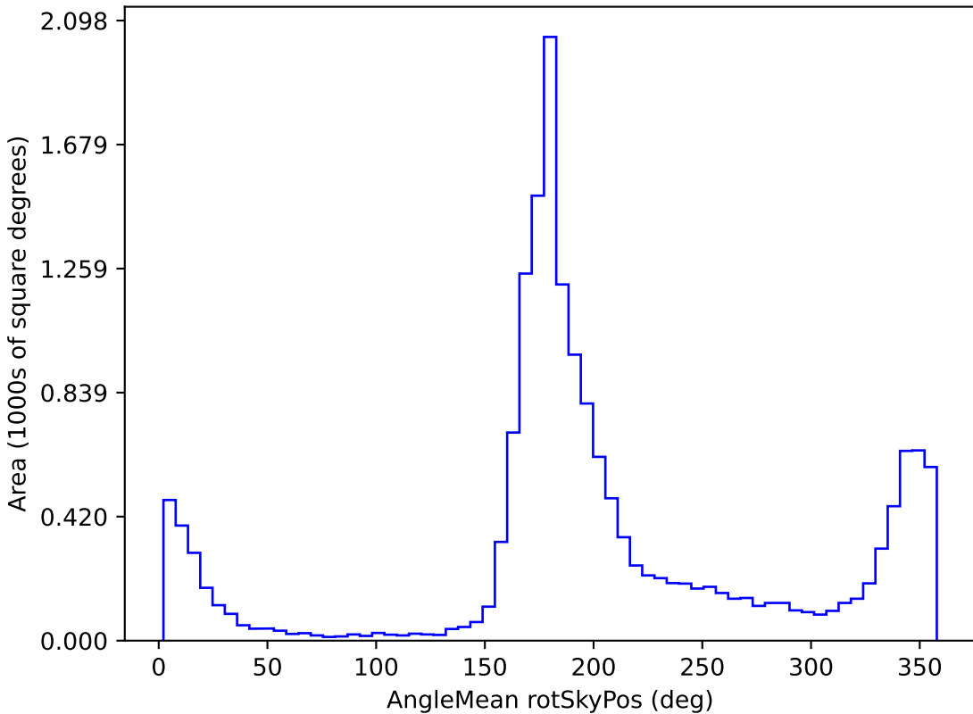
baseline_v2.0_10yrs WFD u band: AngleMean rotSkyPos
