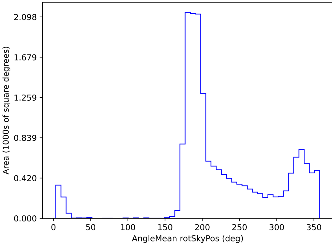
baseline_v2.0_10yrs WFD r band: AngleMean rotSkyPos
