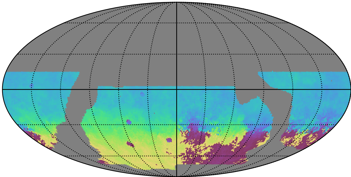
baseline_v2.0_10yrs WFD g band: AngleMean rotSkyPos
