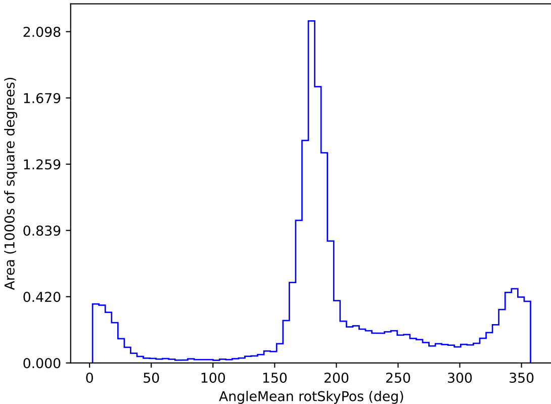
baseline_v2.0_10yrs WFD g band: AngleMean rotSkyPos
