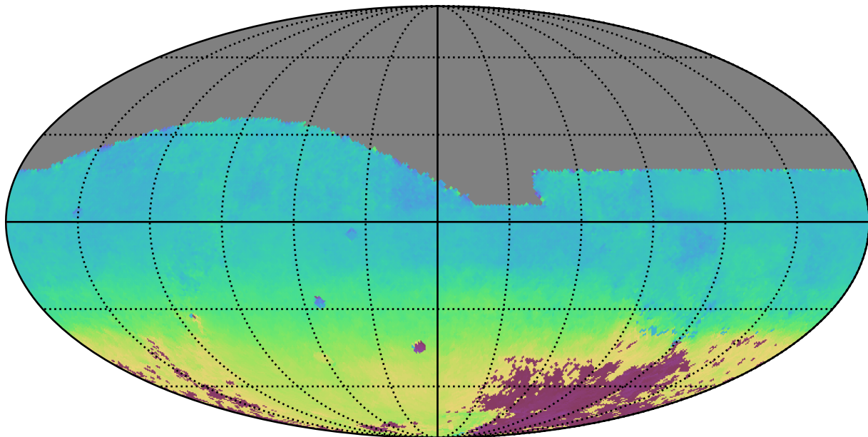
baseline_v2.0_10yrs All sky z band: AngleMean rotSkyPos
