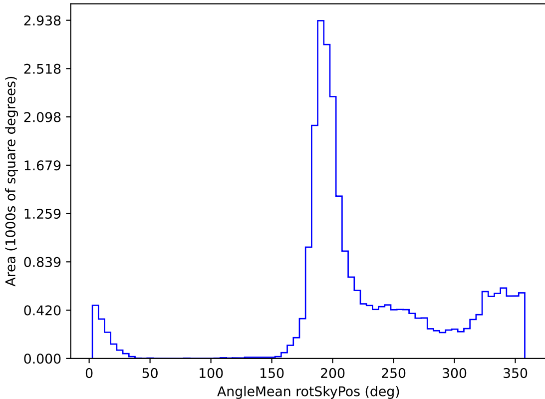
baseline_v2.0_10yrs All sky z band: AngleMean rotSkyPos
