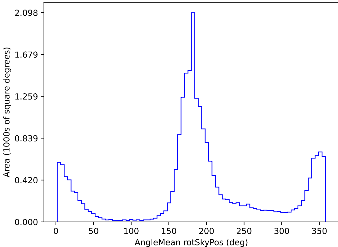
baseline_v2.0_10yrs All sky u band: AngleMean rotSkyPos
