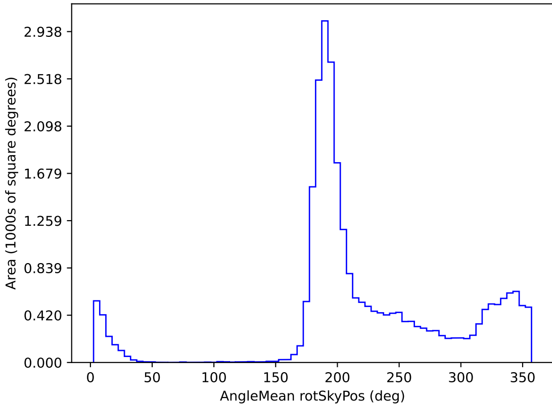
baseline_v2.0_10yrs All sky i band: AngleMean rotSkyPos
