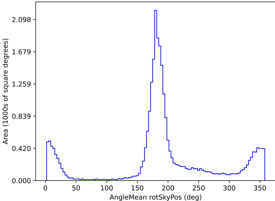
baseline_v2.0_10yrs All sky g band: AngleMean rotSkyPos
