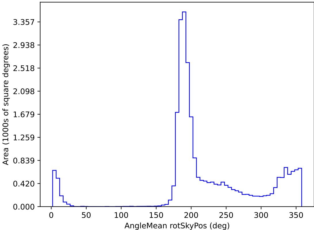
baseline_v2.0_10yrs All sky all bands: AngleMean rotSkyPos
