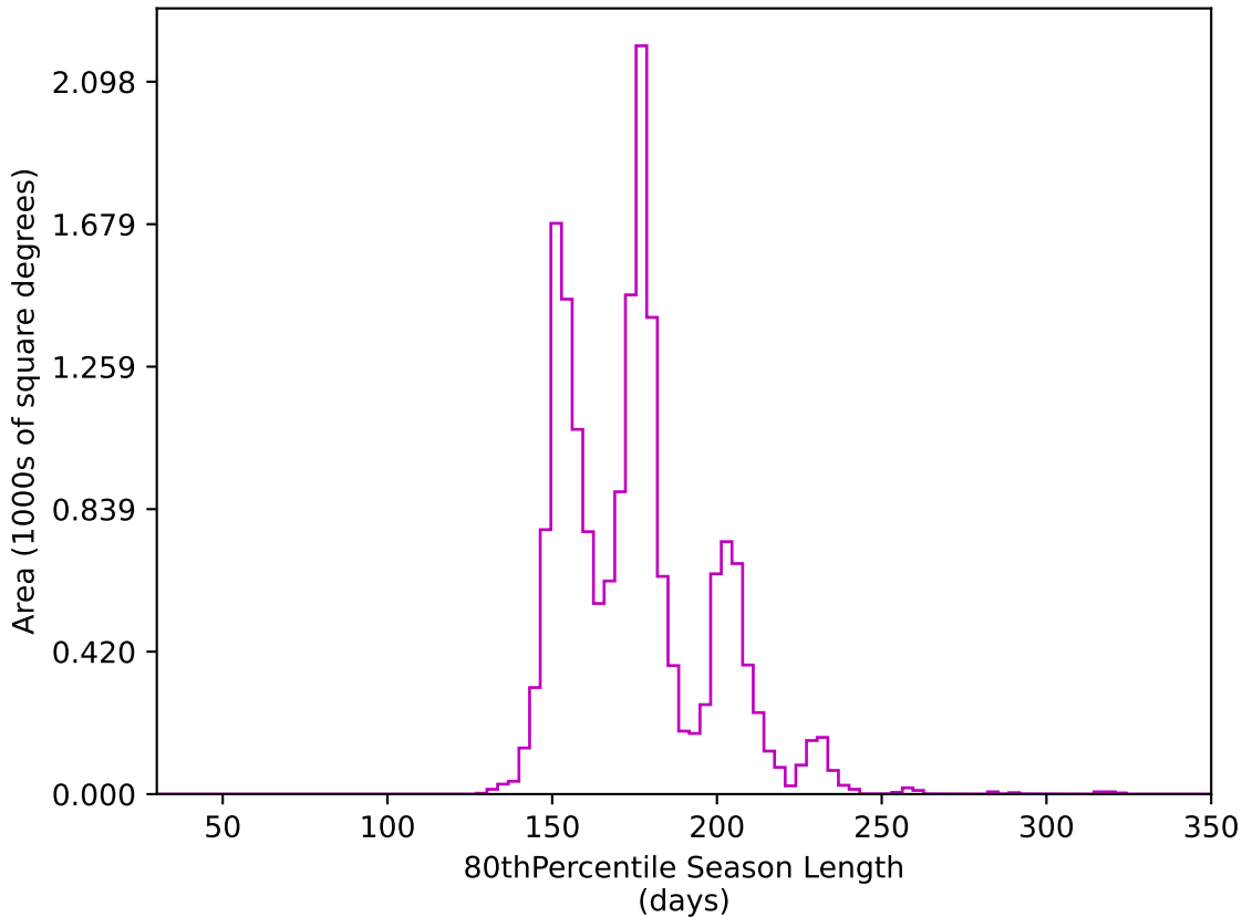
baseline_v2.0_10yrs WFD z band: 80thPercentile Season Length
