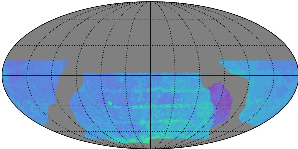
baseline_v2.0_10yrs WFD y band: 80thPercentile Season Length
