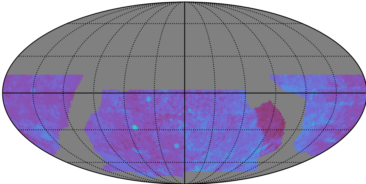
baseline_v2.0_10yrs WFD u band: 80thPercentile Season Length
