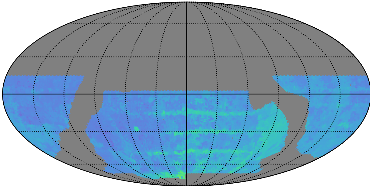
baseline_v2.0_10yrs WFD r band: 80thPercentile Season Length
