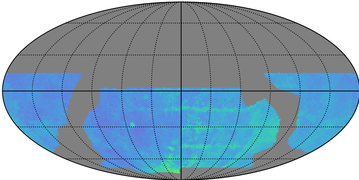
baseline_v2.0_10yrs WFD i band: 80thPercentile Season Length
