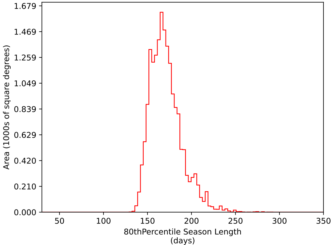
baseline_v2.0_10yrs WFD i band: 80thPercentile Season Length
