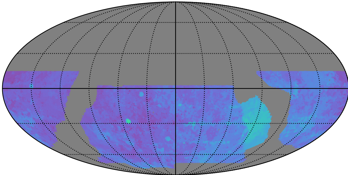
baseline_v2.0_10yrs WFD g band: 80thPercentile Season Length
