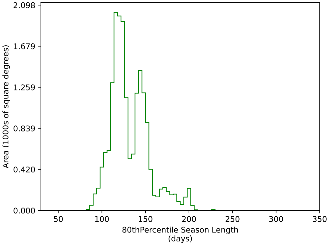
baseline_v2.0_10yrs WFD g band: 80thPercentile Season Length
