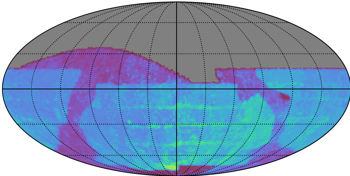
baseline_v2.0_10yrs All sky z band: 80thPercentile Season Length
