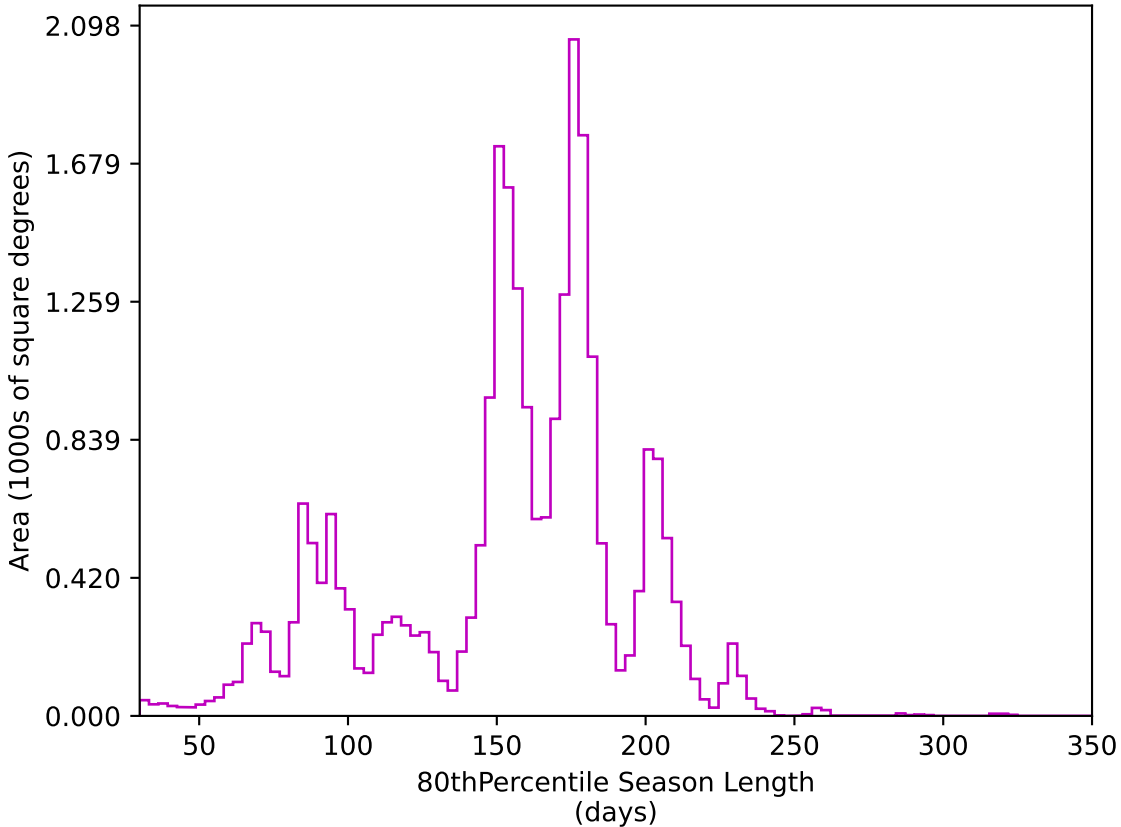
baseline_v2.0_10yrs All sky z band: 80thPercentile Season Length
