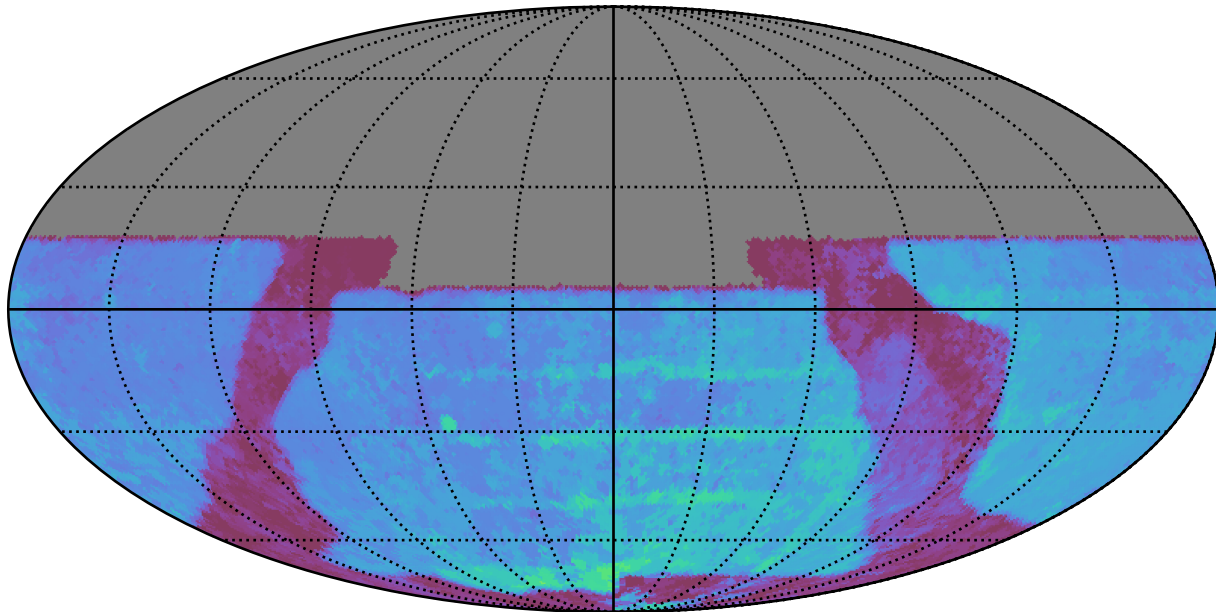
baseline_v2.0_10yrs All sky y band: 80thPercentile Season Length
