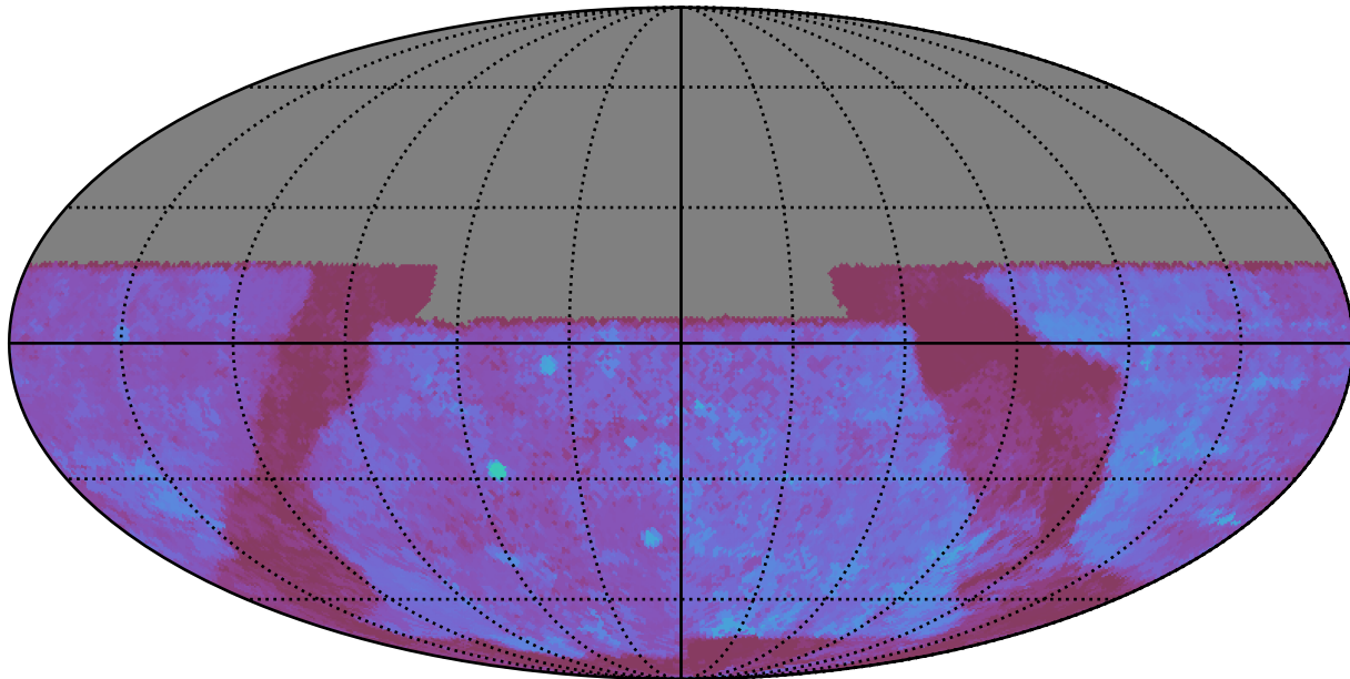
baseline_v2.0_10yrs All sky u band: 80thPercentile Season Length
