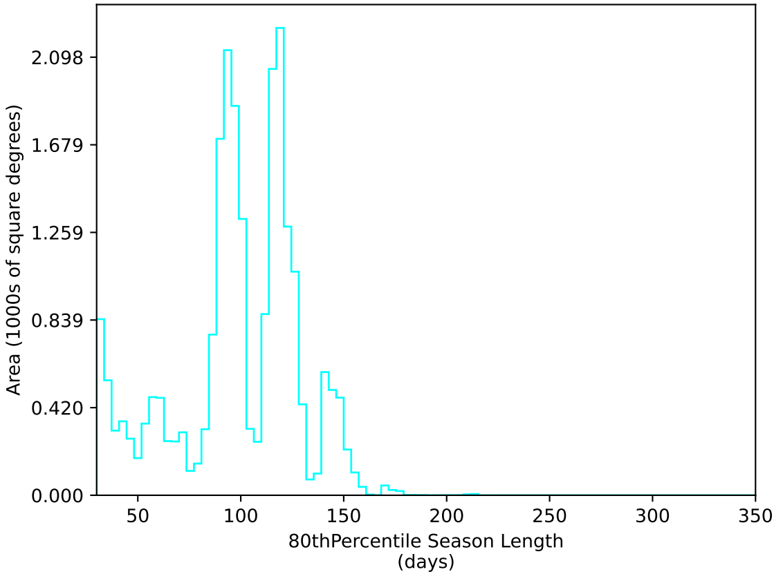
baseline_v2.0_10yrs All sky u band: 80thPercentile Season Length
