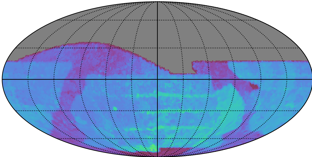
baseline_v2.0_10yrs All sky r band: 80thPercentile Season Length
