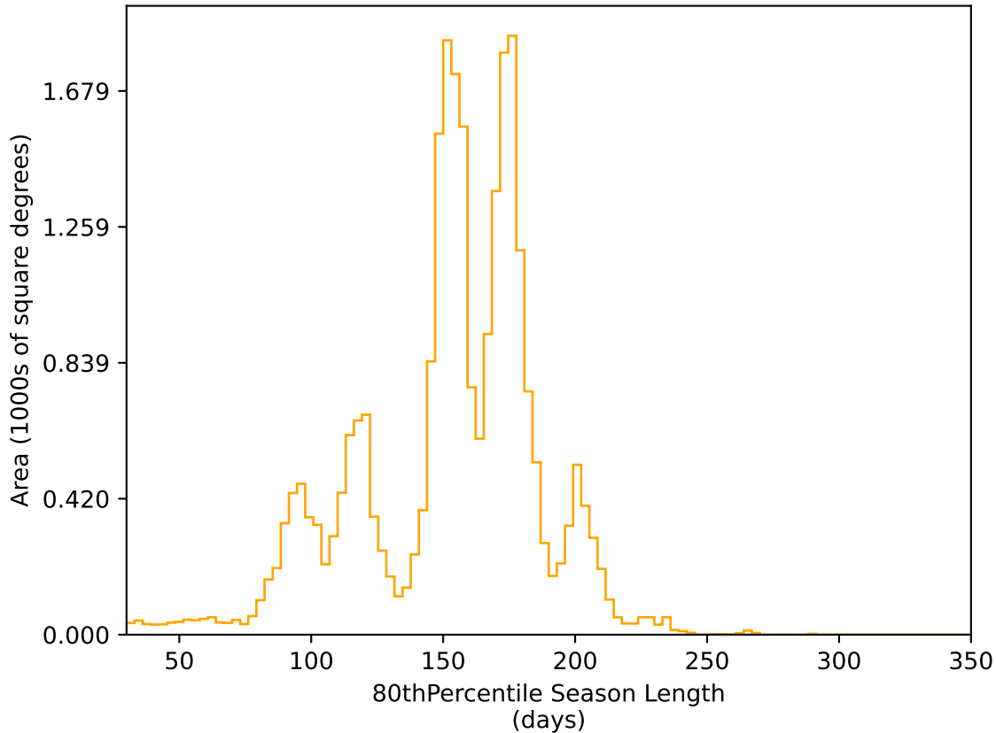
baseline_v2.0_10yrs All sky r band: 80thPercentile Season Length
